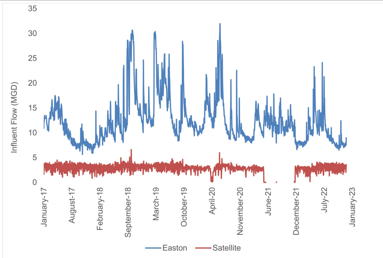
Figure 2 Influent Flow
