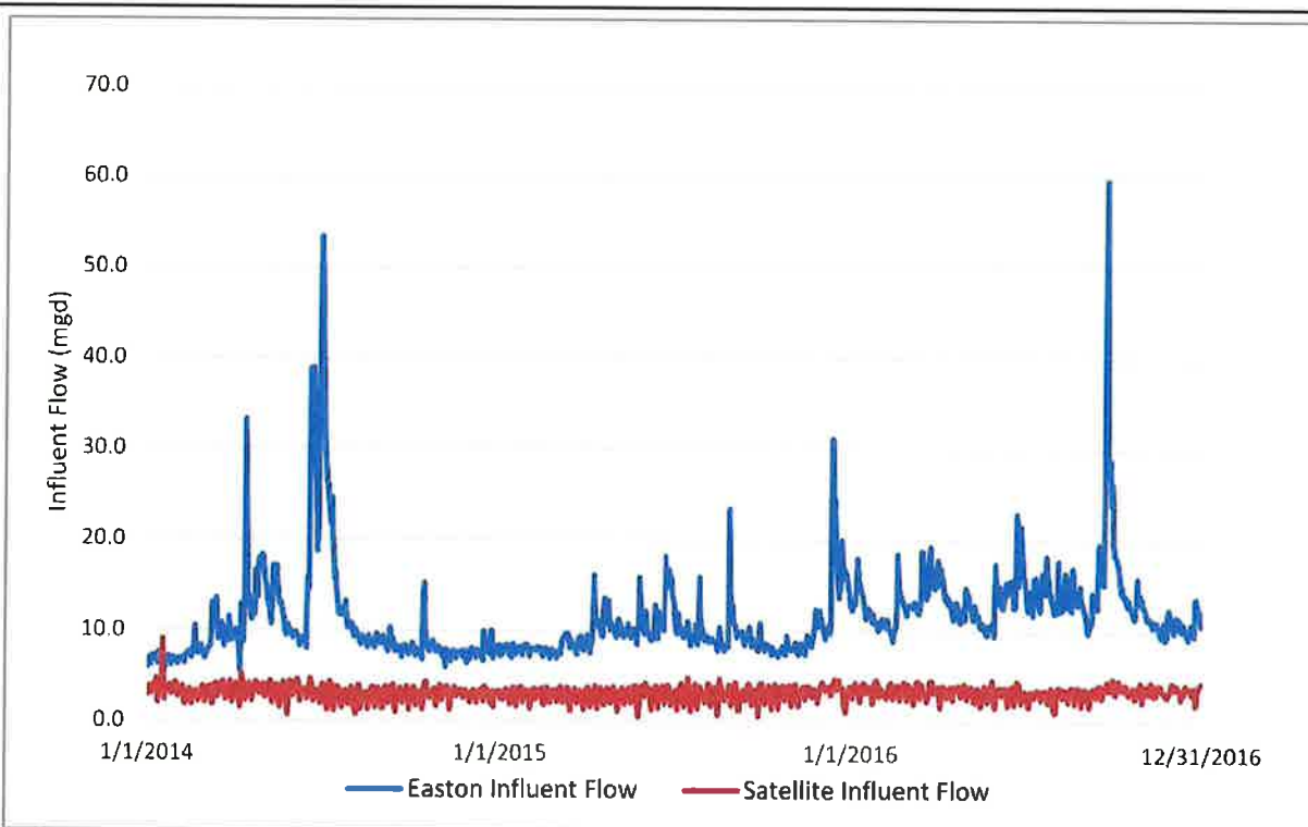
Figure 2 Influent Flow
